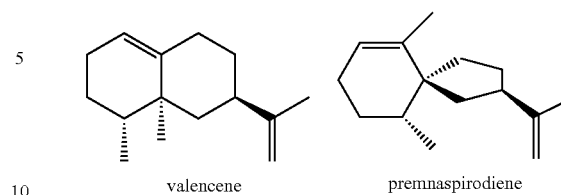
Scheme 3. Structures of valencene and premnaspirodiene.
